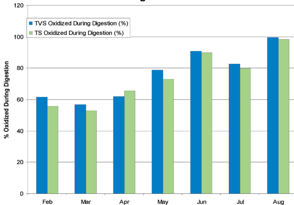
Volatile Solids Destruction Efficiency Before and After Using BIO ENERGIZER®
